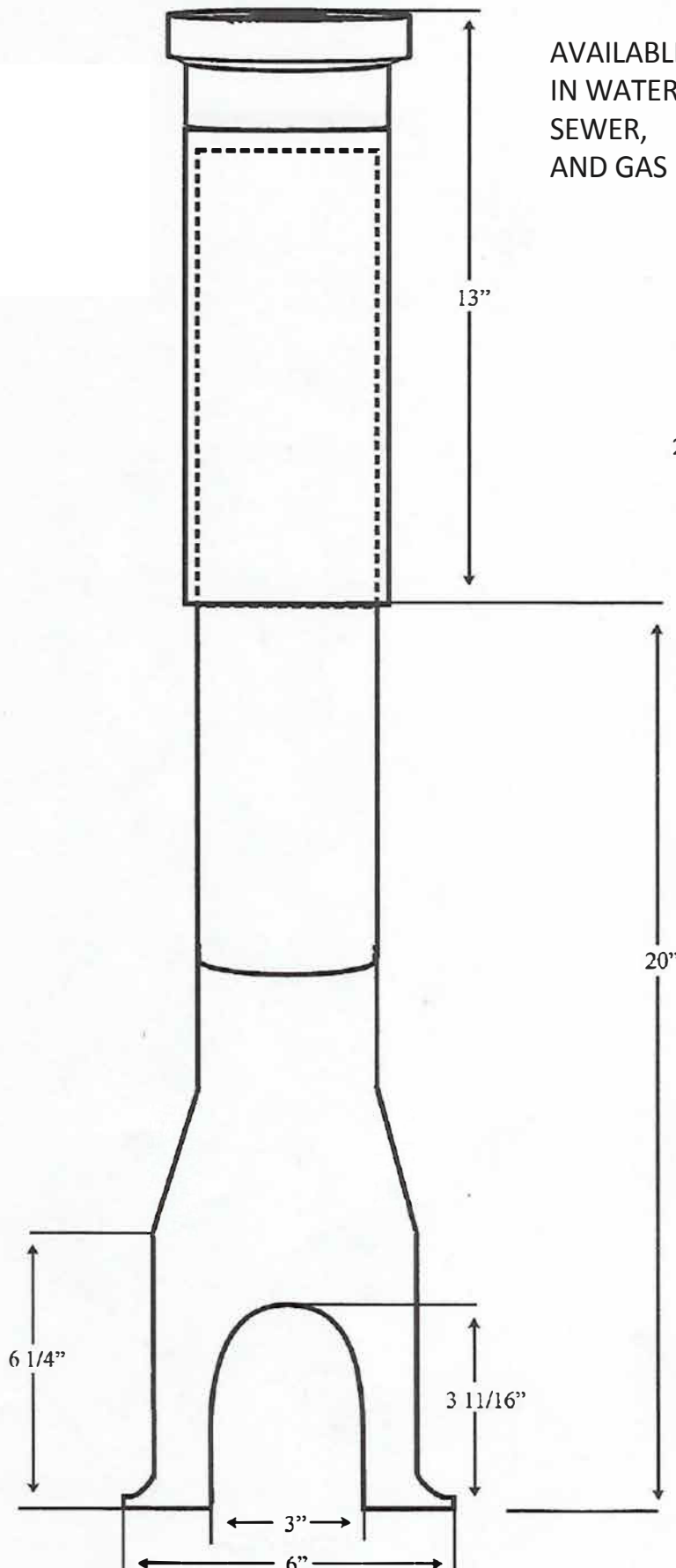
Figure # 3111212PBSA 3" Curb Box Complete Extension Range 18" - 30" Combination Cast Iron/ABS Slip Type Standard Arch
