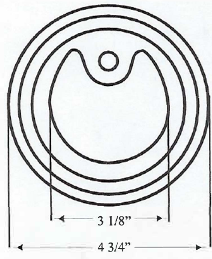
Figure # 3111212PBSA 3" Curb Box Complete Extension Range 18" - 30" Combination Cast Iron/ABS Slip Type Standard Arch
