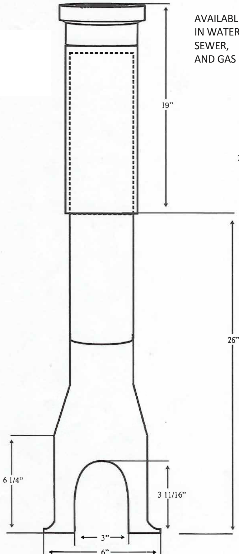
Figure # 311818PBSA 3" Curb Box Complete Extension Range 30" - 42" Combination Cast Iron/ABS Slip Type Standard Arch
