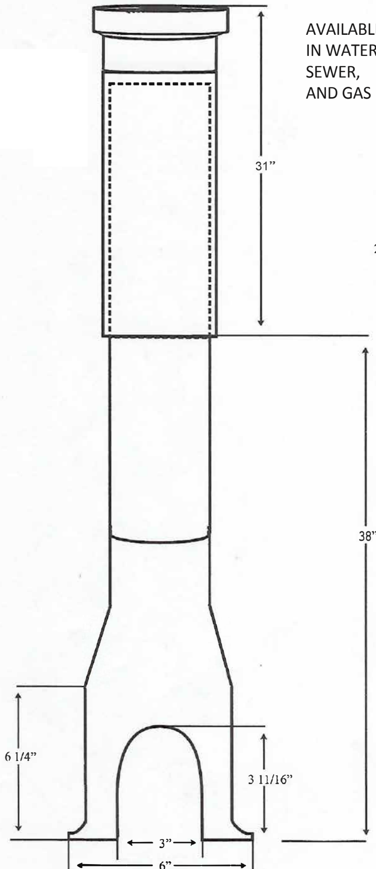
Figure # 3113030PBSA 3" Curb Box Complete Extension Range 42" - 66" Combination Cast Iron/ABS Slip Type
