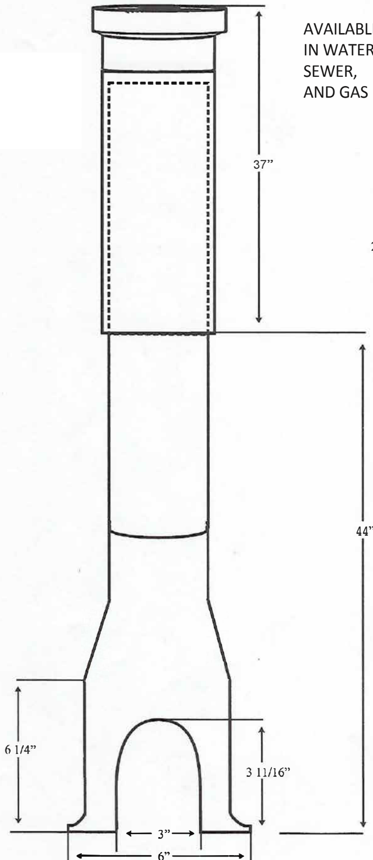
Figure # 3113636PBSA 3" Curb Box Complete Extension Range 48" - 78" Combination Cast Iron/ABS Slip Type
