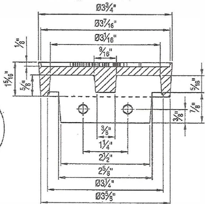
SECTION XX
