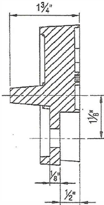
SECTION YY
